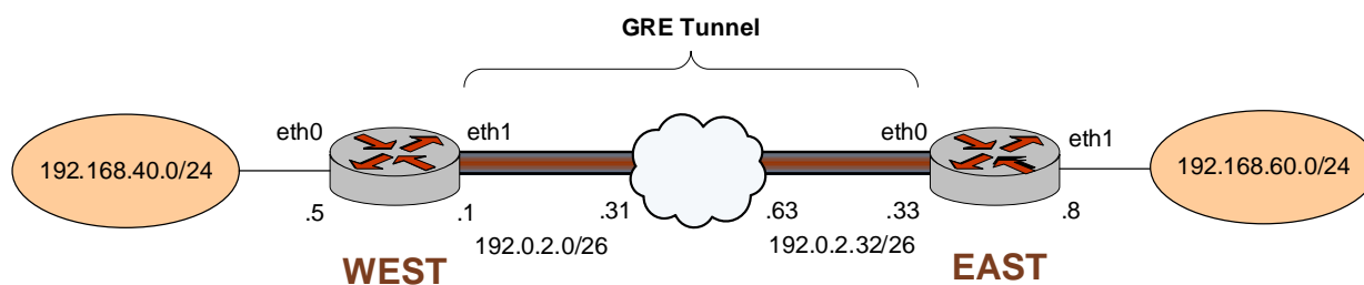
Figure 2-1 Basic GRE tunnel
